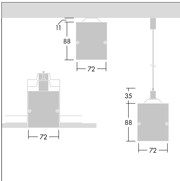
TLG_EQUAL_M_surface_susepended_plasterboard.wmf
