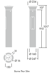
Borne Thor Slim
