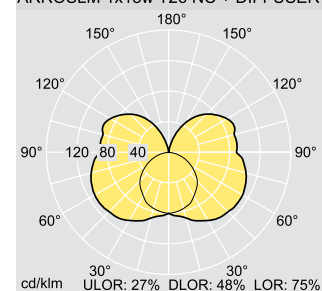
ARROSLM 1x18w T26 NC + DIFFUSER
