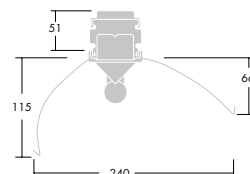
T8 aluminiumreflektor, wall washer 1-rörs
