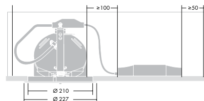
Cruz 160G 35-70W HIT
