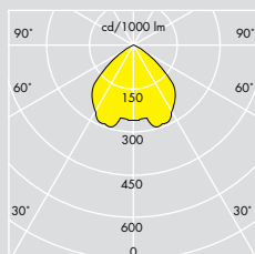
AL315 horisontell HF 2 x 18W TC-DEL ULOR: 0% DLOR: 68% LOR: 68%
