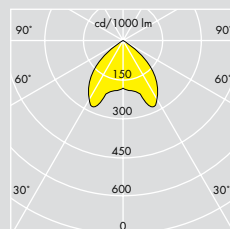
AL350 vertikal HF 2 x 26W TC-DEL ULOR: 0% DLOR: 73% LOR: 73%
