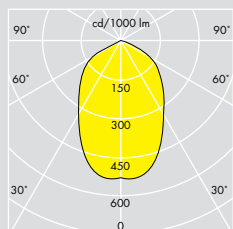
AL220 horisontell HF 1 x 18W TC-DEL ULOR: 0% DLOR: 65% LOR: 65%
